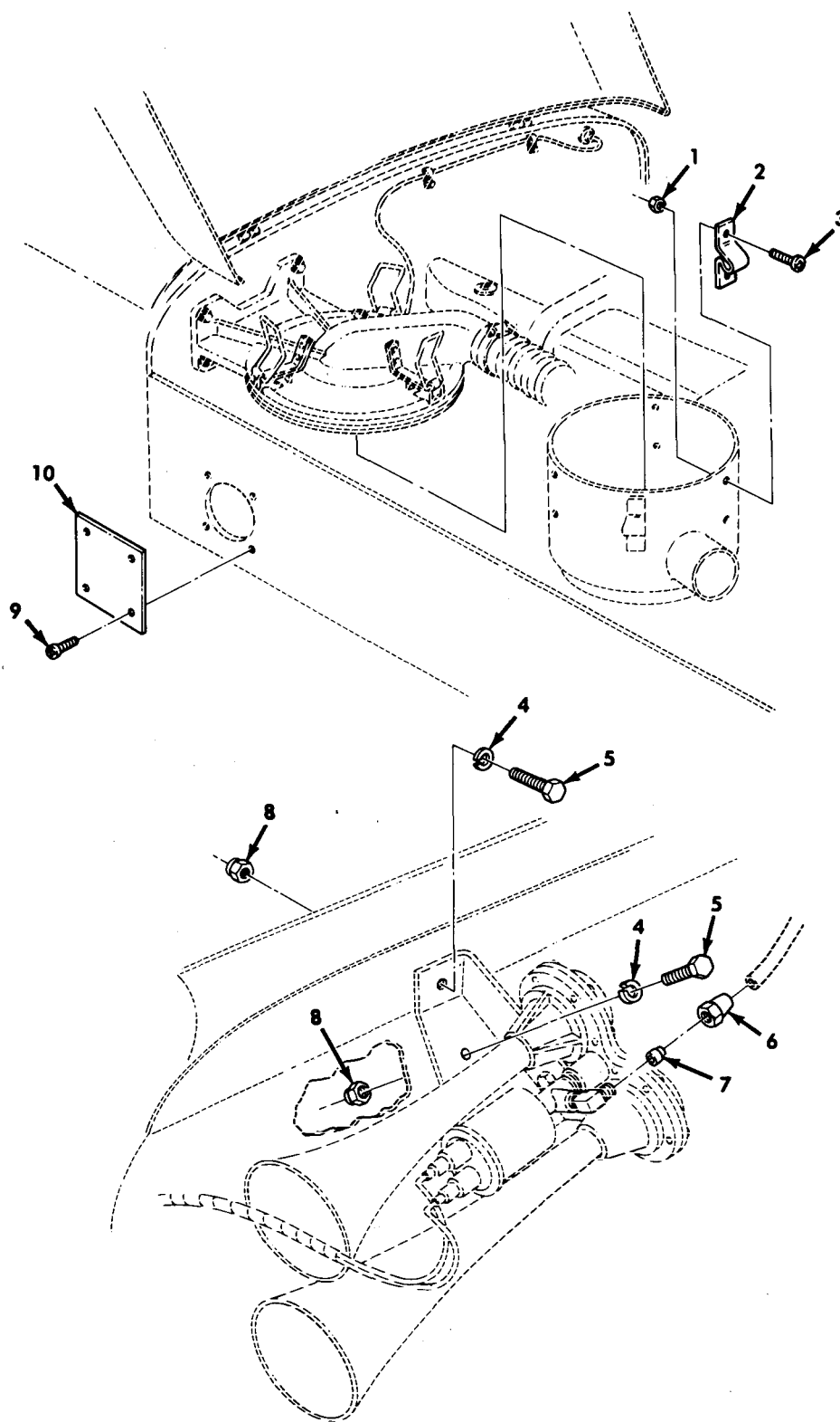
Figure 274. Cover Plate, Latch, and Related Parts, Cab and Engine Swingfire Heater Kit.
