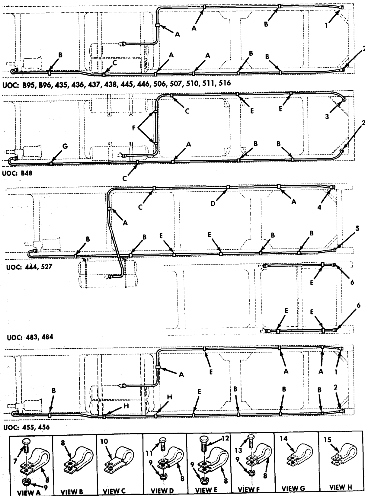
Figure 103. Rear Coupling Air Lines and Mounting Hardware.
