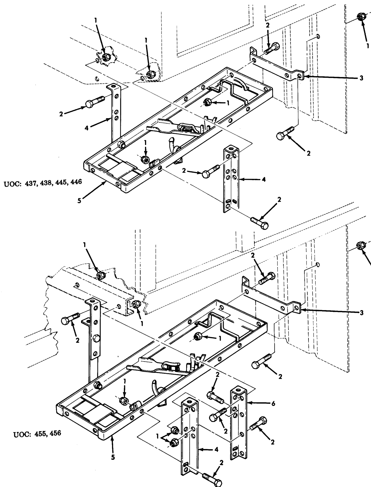
Figure 321. Pioneer Tool Bracket Kit, Cargo.
