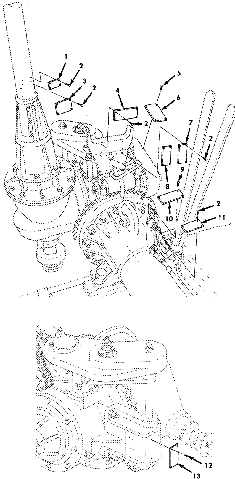
Figure 256. Data Plates, Earth Boring Machine.
