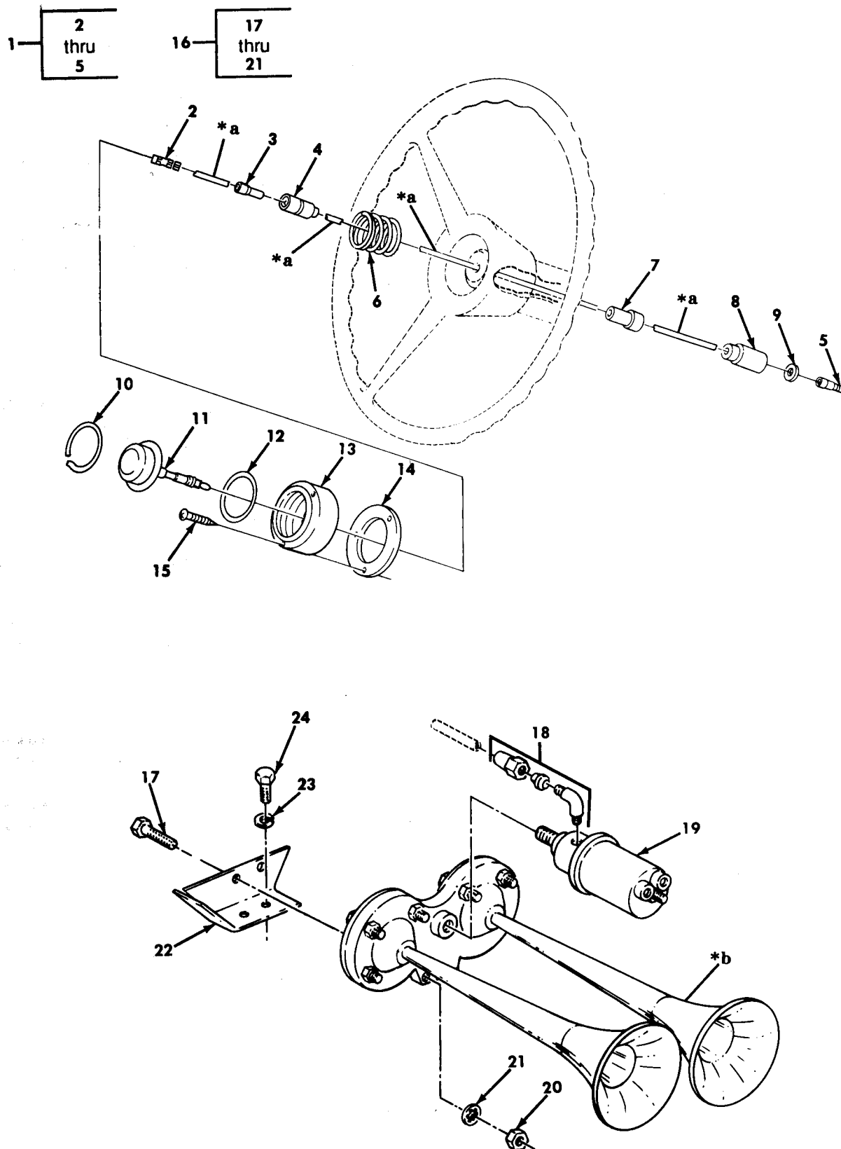
Figure 55. Horn Button and Air Horn Assembly.
