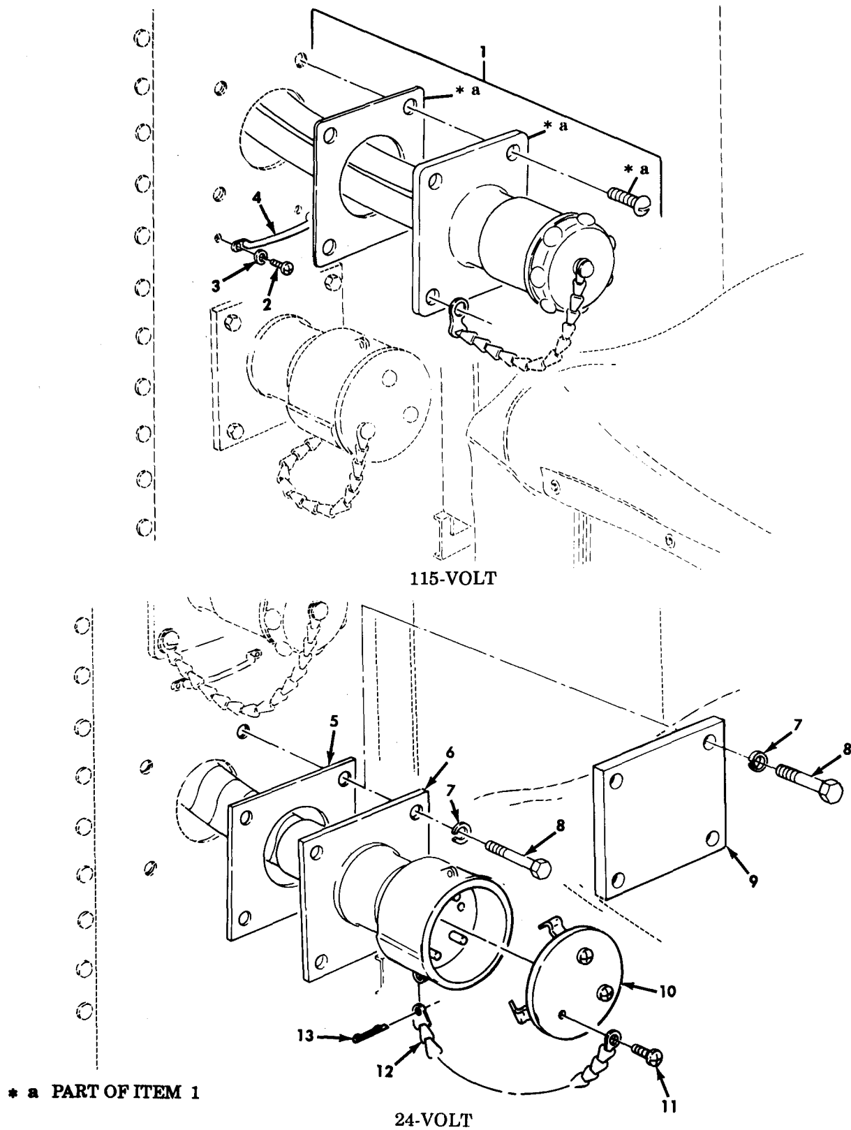
Figure 189. 115-Volt and 24-Volt Receptacle Harness and Related Parts.
