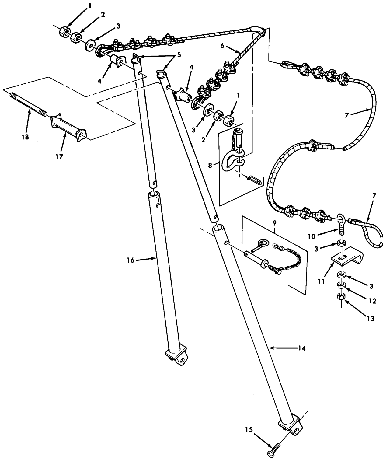
Figure 295. A-Frame Kit.
