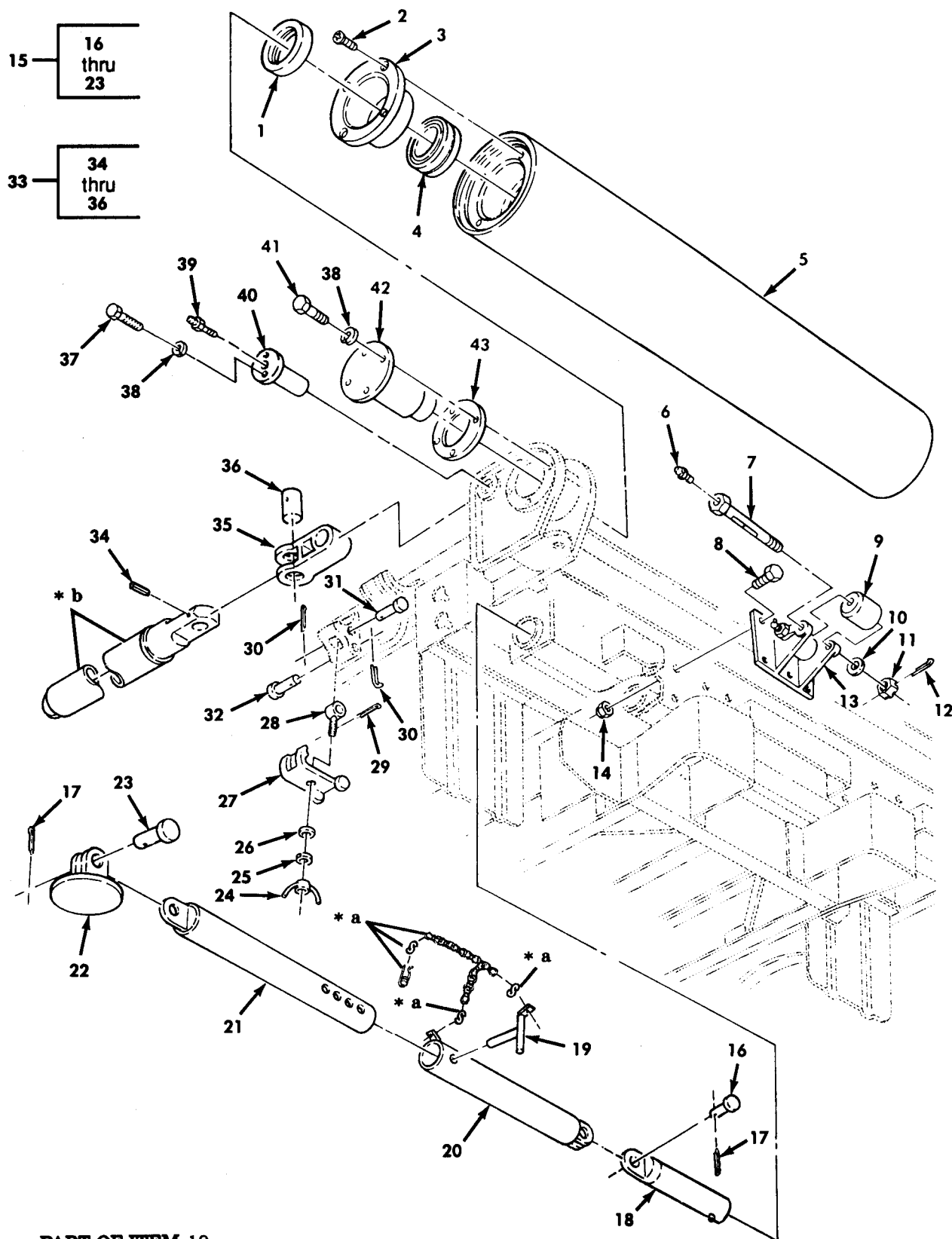
Figure 216. Stiffleg Jack, Gin Pole, and Roller Assemblies.
