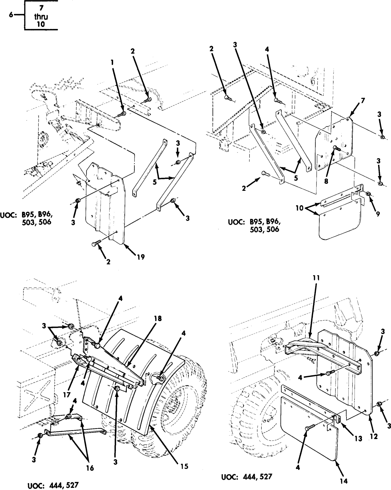
Figure 136. Splash Guards.
