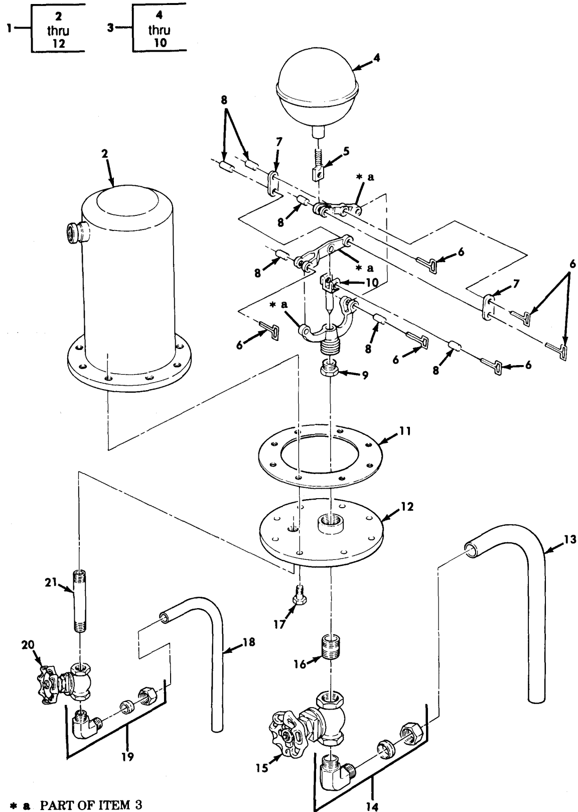
Figure 176. Automatic Dump Valve and Sump Assembly.
