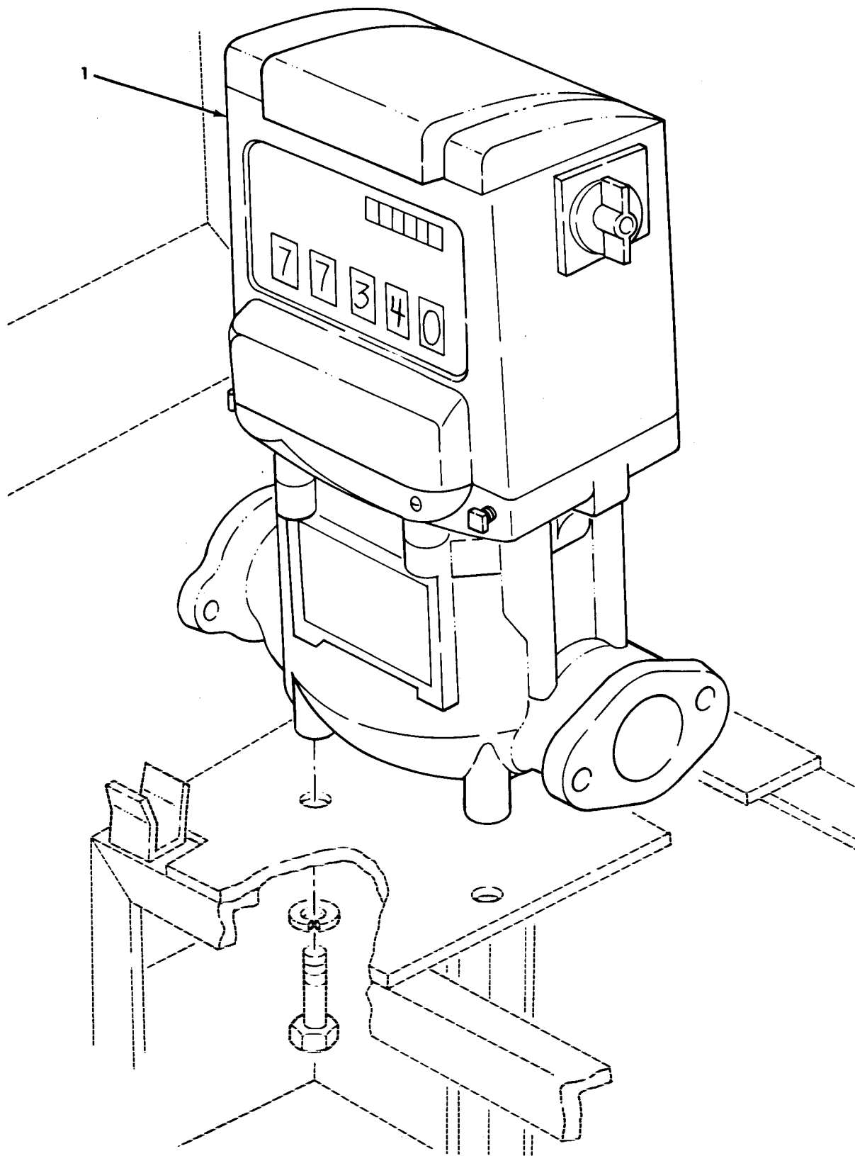
Figure 328. Meter.
