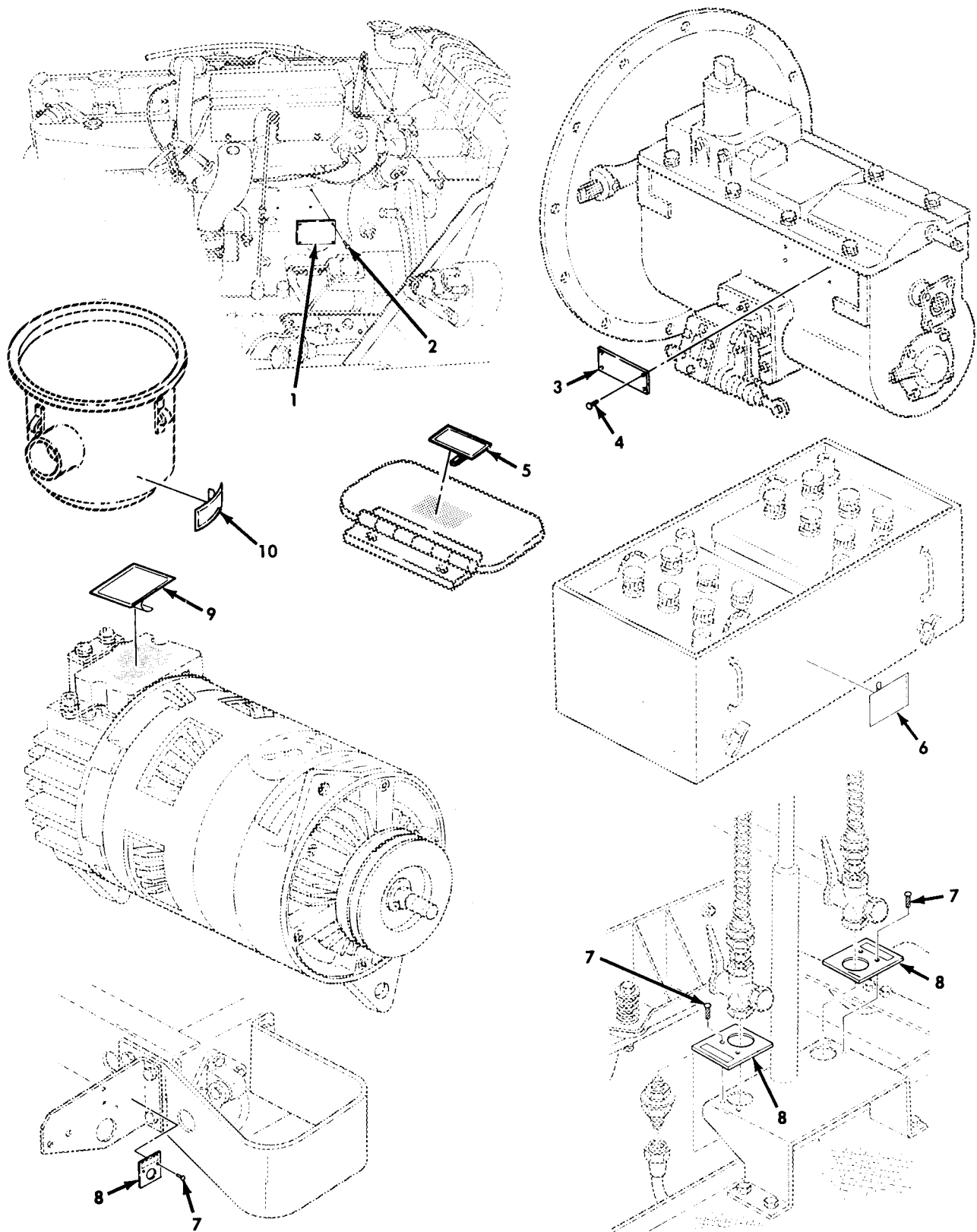
Figure 250. Data Plates.
