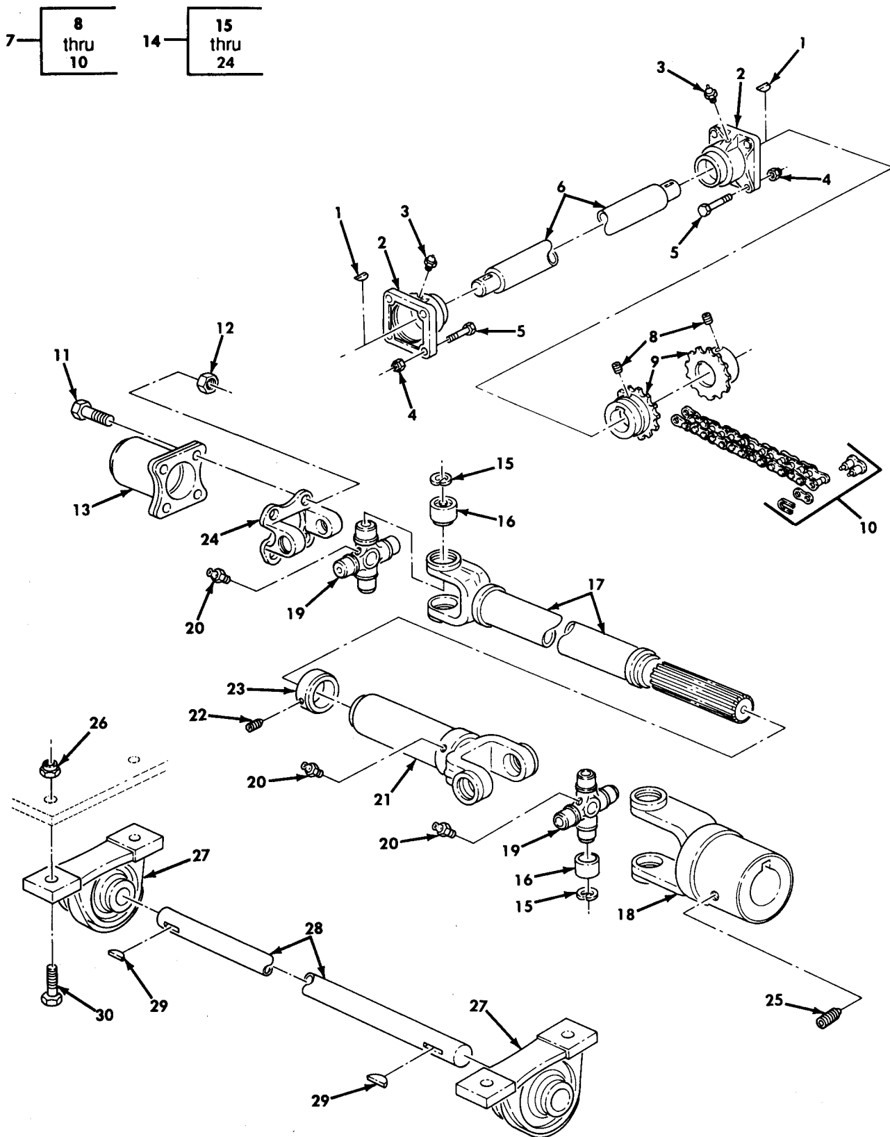
Figure 162. Drive Shaft Assemblies.
