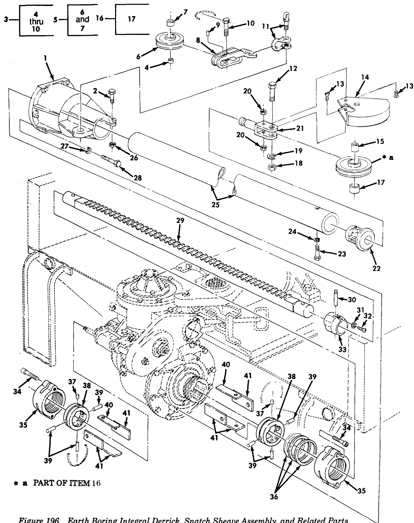
Figure 196. Earth Boring Integral Derrick, Snatch Sheave Assembly, and Related Parts.
