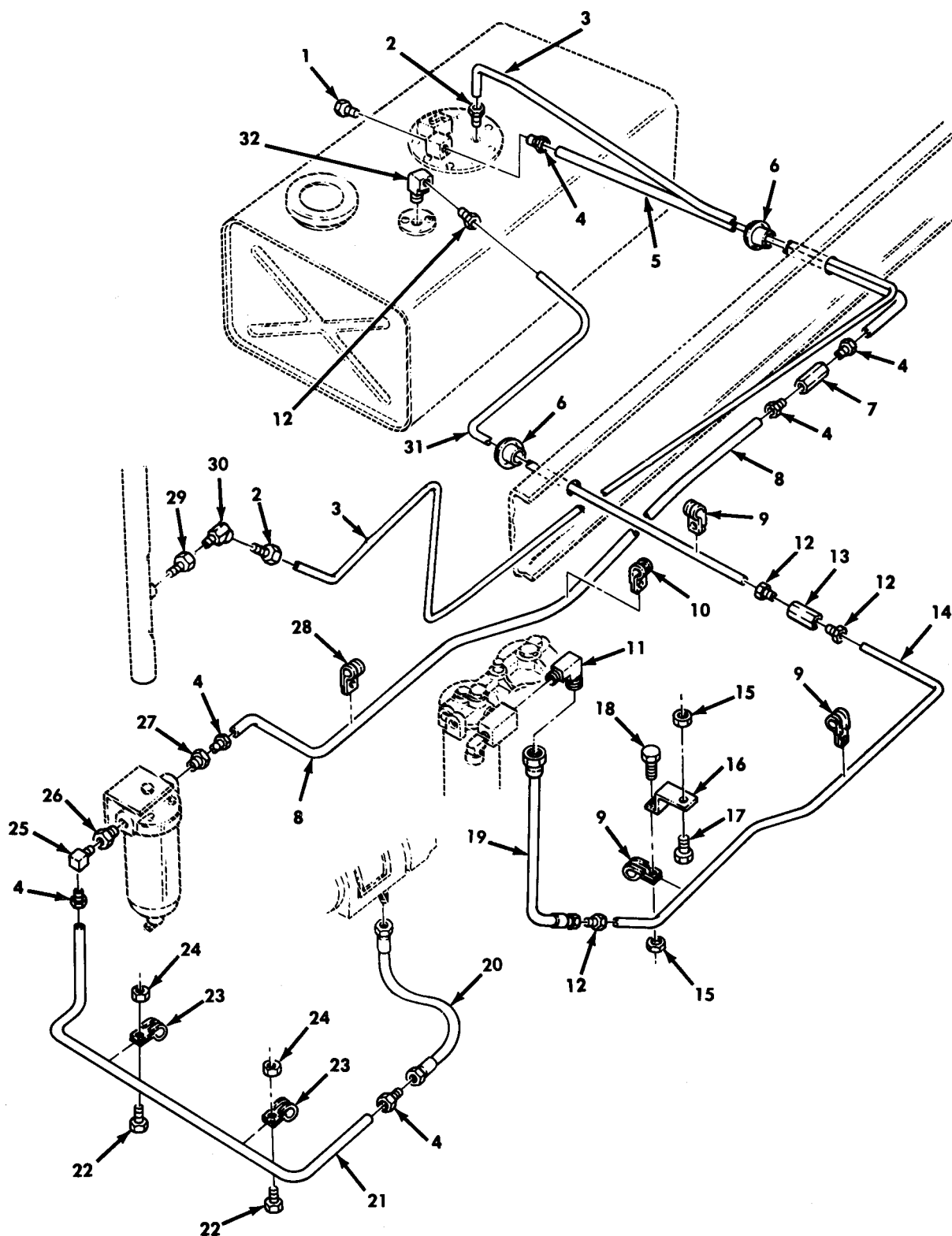
Figure 25. Fuel Lines and Related Parts.
